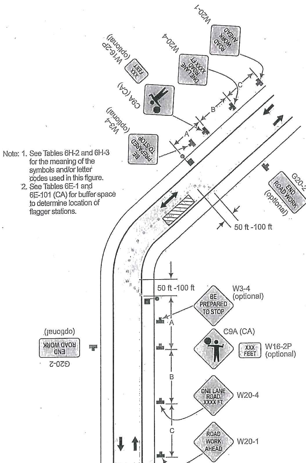
Typical Application 10
